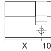
Haif cylinder with single entry X=30mm~60mm
