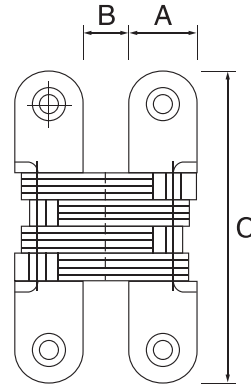
Concealed hinge
